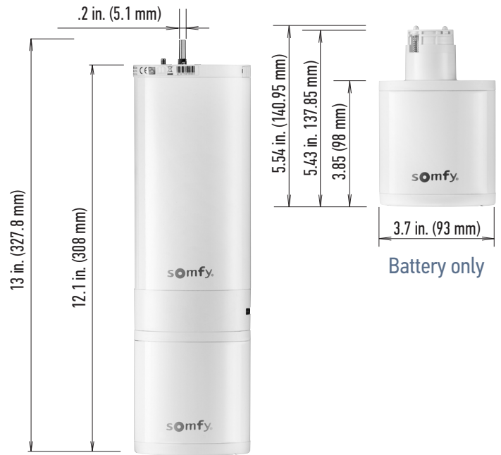
Motor and Battery
